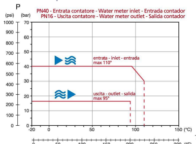
TemperaturePression
